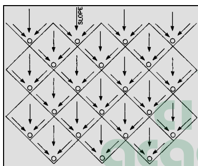
Figure 2.1: Field Layout for Negarim Micro-Catchments
