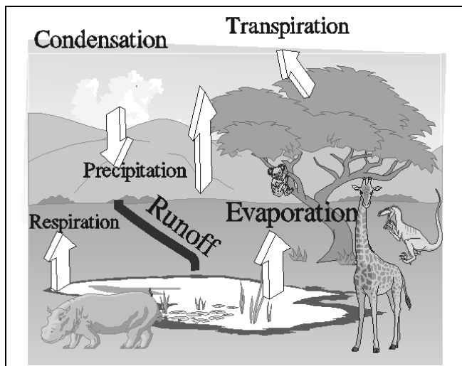
Figure 1.1: The Water Cycle
