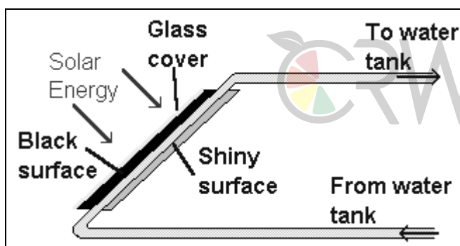
Figure 1.2: Simple Solar Water-Heating Device
