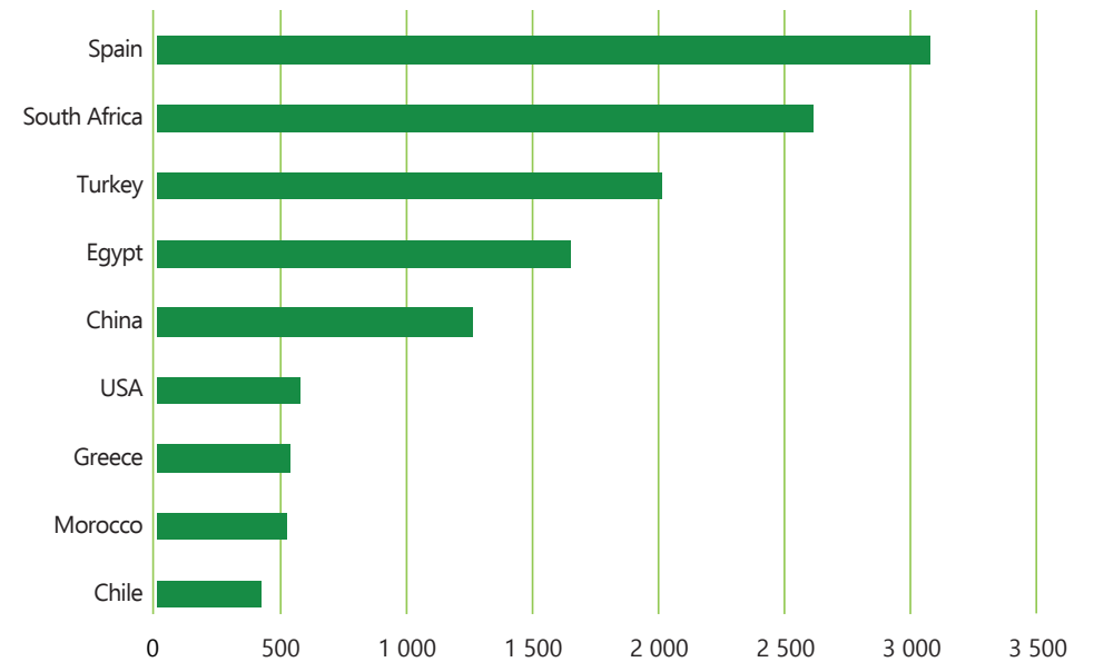
World Fresh Citrus Exports 2022/2023 (Thousand Tons)
